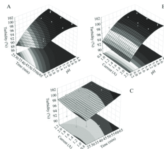
Figure 4. Response surface of experimental data for turbidity reduction. Optimization equation: \hat{y}_{turbidez} (\%) = 98.03 - 2.88x_1 + 1.20x_2 - 0.06x_3 - 1.44x_1^2 + 0.04x_2^2 + 0.21x_3^2 + 1.29x_1 \cdot x_2 - 0.11x_1 \cdot x_3 - 0.28x_2 \cdot x_3 .
