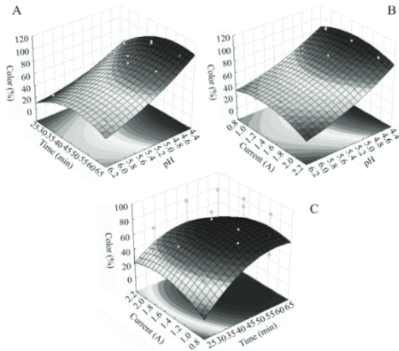
Figure 5. Response surface of experimental data for color reduction. Optimization equation: \hat{y}_{cor}(\%) = 61.84 - 25.58x_1 + 11.77x_2 - 1.97x_3 - 5.97x_1^2 + 11.20x_2^2 + 7.22x_3^2 - 4.53x_1 \cdot x_2 - 1.54x_1 \cdot x_3 - 5.10x_2 \cdot x_3 .
